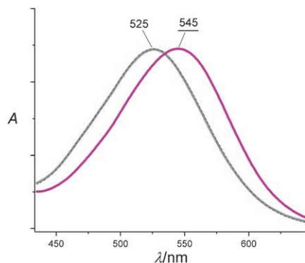
Figure 2. Absorption spectra of the wild-type (dotted line), A115R mutant (gray solid line), and A178R mutant (pink solid line) PRs at pH 7.0. The \lambda_{\max} value is red shifted by 20 nm for A178R.
